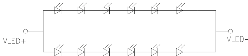
LED circuit diagram
